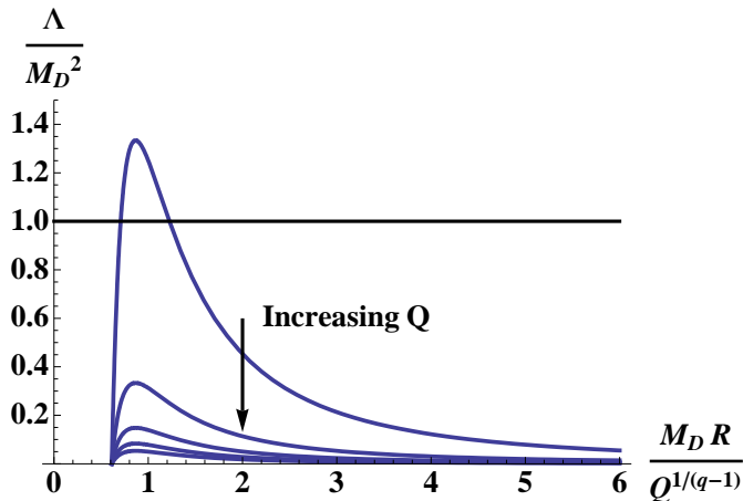
Figure 4. Extrema of the radion potential are located at the intersection of each curve (eq. (2.16) for \{p = 2, q = 2\} ) with a line of fixed \Lambda . There is only one intersection at \Lambda = 0 and zero, one, or two intersections at \Lambda > 0 . When there are two intersections, the first corresponds to a minimum (referred to as R_- or \phi_- ) and the second to a maximum (referred to as R_+ or \phi_+ ). Note that the location of the first intersection is relatively independent of \Lambda .
