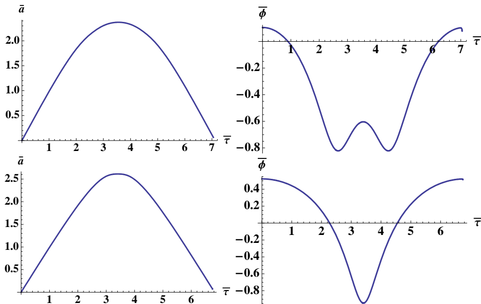
Figure 7. The oscillatory solutions for timelike \tau with \Lambda = 0 , Q = 1 , p = 5 , and q = 2 . The solutions for \bar{a}(\bar{\tau}) (left in each row) and \bar{\phi}(\bar{\tau}) (right) describe the spacetime between two event horizons of the D -dimensional geometry (see figure 6). Event horizons are located at the zeros in a . The top panel shows the oscillatory solutions with 4 nodes, generated from the initial condition \phi_0 \simeq .105 . The bottom panel shows the oscillatory solution with 2 nodes generated from the initial condition \phi_0 \simeq .523 . A scan over initial conditions reveals that these are the unique non-singular solutions.
