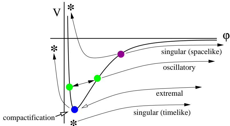
Figure 5. A sketch of the solutions for \Lambda = 0 with a flat or open FRW ansatz for the p + 2 -dimensional metric. Beginning from stationary points \dot{\phi} = 0 (filled circles), the evolution is in the potential V for \tau timelike (trajectories above the potential) or -V for \tau spacelike (trajectories below the potential). Singularities along a trajectory are denoted by an asterisk. The compactification solution sits at the potential minimum for all \tau . The singular (timelike and spacelike), extremal, and oscillatory solutions all have a region where \tau is spacelike and \phi \rightarrow \infty , universally approaching the attractor solution eq. (4.14). Continuing across an arbitrary stationary point to a region where \tau is timelike will result in a spacelike singularity. There are special stationary points from which \phi oscillates about the potential minimum (indicated by the double arrows on the oscillatory trajectory). For a flat FRW metric ansatz, there are solutions where \tau is everywhere spacelike, and the field interpolates between the potential minimum and \phi \rightarrow \pm\infty . Solutions without a stationary point are always singular (timelike).
