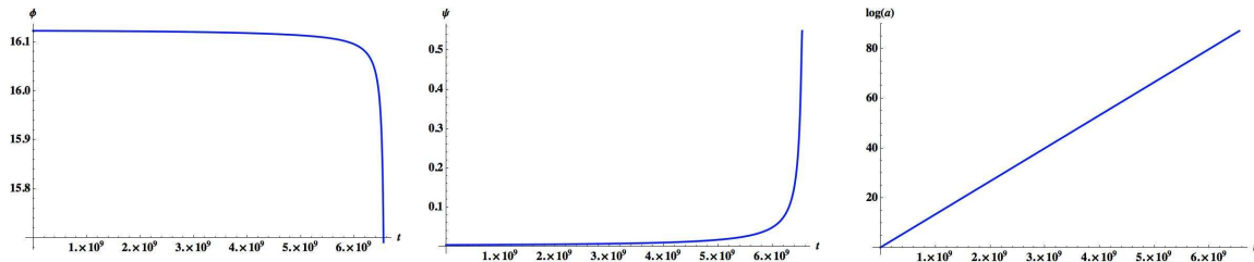
Figure 24. Numerical evolution for the potential in the right panel of figure 22. The parameters specifying the potential are \{q = 2, n = 6, Q = 3651.5, \Lambda = 1 \times 10^{-7}, \tilde{m} = 1.32 \times 10^{-7}, \xi_1 = .199, \xi_2 = -1, \lambda = 3.6 \times 10^{-6}\} . The Euclidean compactification solution places the field near the maximum of the potential in the \phi -direction near \psi = 0 . We choose the initial conditions to be \{\phi_0 = 16.122, \psi_0 = .003\} , which yields approximately 90 e -folds of inflation.
