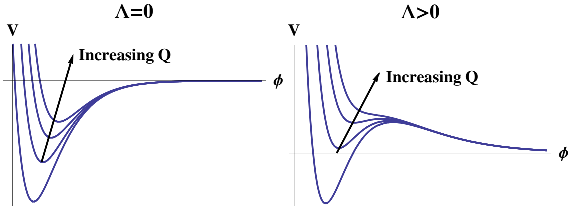
Figure 3. The radion potential eq. (2.15) with \Lambda = 0 (left) and \Lambda > 0 (right). In each plot, a number of potentials at fixed \Lambda are shown with successively larger values of Q from bottom to top. For \Lambda = 0 the potential always has a negative minimum and approaches zero from below as \phi \rightarrow \infty , while for \Lambda > 0 there can exist a minimum of negative, zero, or positive energy and the potential approaches zero from above at large \phi .
