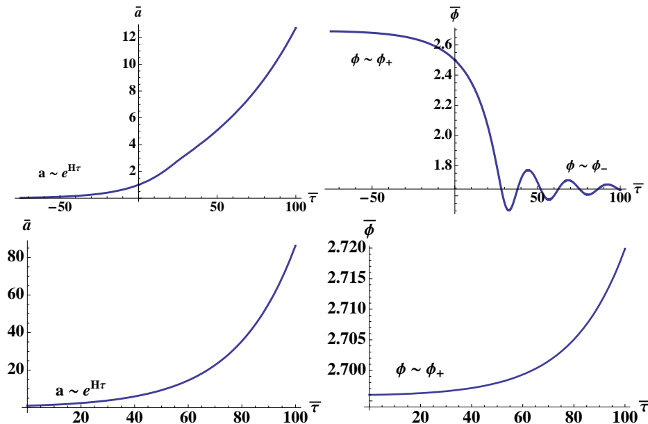
Figure 14. An example of the Nariai solution for p = 2 , q = 2 , Q = 3.2 , and \Lambda/M_D^2 = .1 . The field evolves from the potential maximum to either \phi_- (top) or \phi \rightarrow \infty (bottom) while the scale factor a monotonically increases. The two solutions are matched across the event horizon of the D -dimensional geometry located at \tau = -\infty . This connects the contracting portion of a D -dimensional de Sitter space to a flat p + 2 -dimensional FRW universe that asymptotically has positive vacuum energy.
