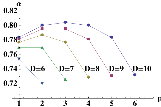
Figure 16. The value of \alpha (eq. (6.15)), the ratio of the instanton action to the D -dimensional de Sitter action, for fixed D and various p in the limit of small Q . Larger values of \alpha correspond to a faster nucleation rate. Circles, squares, diamonds, triangles, and inverted triangles are for D = 10, 9, 8, 7, 6 respectively. In each case, p can range from 1 to D - 2 . The value of \alpha peaks at a value of p dependent on the total dimensionality.
