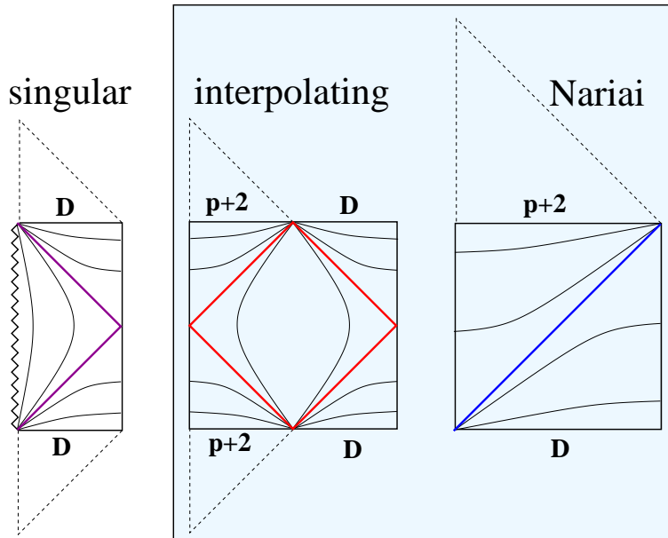
Figure 12. Causal diagrams for \Lambda > 0 solutions with an asymptotically D -dimensional region and a radion potential that has a positive or zero minimum. Surfaces of constant \tau are shown as the light solid lines. Starting from the left, we show the singular, interpolating, and Nariai solutions. In the interpolating solution, future/past infinity is split between non-singular regions of different effective dimensionality (the dimensionality is labeled D or p + 2 ). When the minimum has zero energy, the p + 2 -dimensional parts of future infinity is null (denoted by the dashed “hat”). The Nariai solution connects the contracting portion of a D -dimensional de Sitter space to a non-singular p + 2 -dimensional flat FRW universe across an event horizon. The horizons are in each case color coded with the stationary points of the radion field in figure 9. We highlight the solutions relevant for dynamical compactification in the shaded box.
