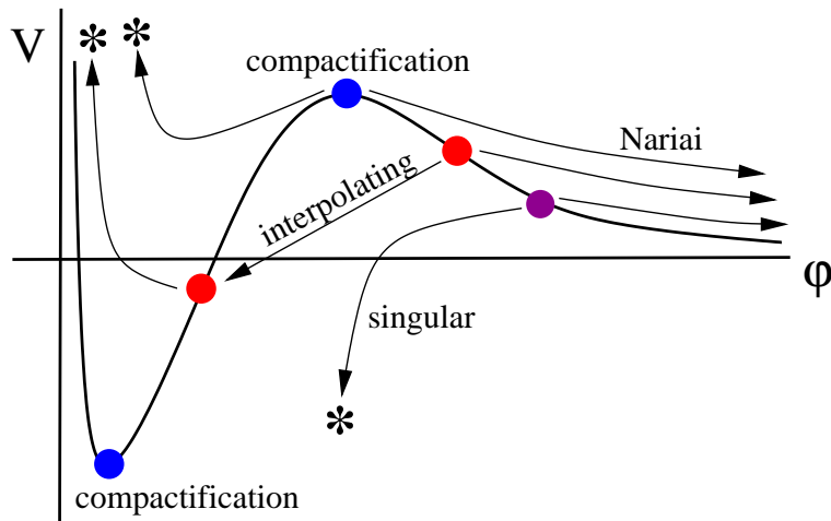
Figure 9. A sketch of the solutions for \Lambda > 0 when the radion potential has a negative energy minimum. Motion above the potential occurs in a region where \tau is a timelike variable, and motion below in regions where \tau is a spacelike variable. An asterisk denotes the occurrence of a curvature singularity along the trajectory. Non-singular stationary points are denoted by the filled circles. All of the solutions contain a singularity except for the compactification solutions that sit at the critical points of the potential for all \tau . At the minimum, an AdS_{p+2} \times S^q geometry results, and at the maximum a dS_{p+2} \times S^q geometry results. For an open FRW ansatz, the interpolating solution has two non-singular stationary points and connects \phi \rightarrow \infty to a region containing a spacelike singularity. All other choices for the location of the stationary points will lead to a timelike singularity. In either of these cases, the D -dimensional solution approaches de Sitter as \tau \rightarrow \infty . For a flat FRW ansatz, the Nariai solution connects regions interpolating between \phi_+ and \phi \rightarrow \pm\infty over an infinite range in \tau . The Nariai solution has a stationary point at \phi_+ , but the geometry is distinct from the compactification solution (although the near-horizon geometry of the Nariai solution is locally dS_{p+2} \times S^q ).
