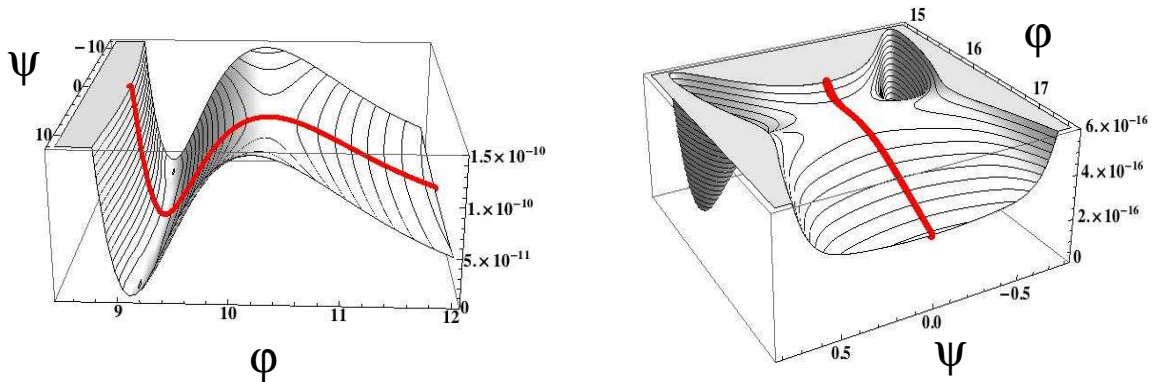
Figure 22. Two models of inflation arising from the potential eq. (8.4). In both cases, the \psi field becomes destabilized between the minimum and maximum of the potential along the \phi direction (the profile along \psi = 0 is shown as the solid line). This can either drive (left) or end (right) an epoch of slow-roll inflation. For the potential on the left, there exists an interpolating solution, which naturally sets the initial conditions near \psi = 0 . Inflation then occurs as the field rolls in the \psi direction. For the potential on the right, there is no interpolating solution, but the Euclidean compactification solution can set the initial conditions for the field very near the potential maximum. Inflation occurs as the field rolls in the \phi direction, eventually ending when the field falls into one of the minima in the \psi direction.
