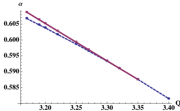
Figure 18. The shaded region of the \alpha versus Q plot of figure 17, in which the radion potential has a positive minimum and the Euclidean compactification (dashed line) and interpolating (solid line) solutions exist. As Q is increased, the instanton endpoints approach the potential maximum, and the value of \alpha for the interpolating solution approaches that for the compactification solutions from above. When it exists, the interpolating solution always makes the dominant contribution to the decay rate.
