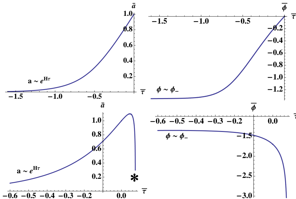
Figure 8. The extremal solutions connecting \phi_- and \phi \rightarrow \infty (top panel) and \phi_- and \phi \rightarrow -\infty (bottom panel). In the bottom panel, there is a singularity at finite \tau when a reaches a second zero, denoted by the asterisk. Near \tau \rightarrow -\infty , the field approaches the potential maximum, and a approaches an exponential. Event horizons of the D -dimensional geometry are located at \tau = -\infty , where the two types of solutions in the top and bottom panels (going to \phi = \pm\infty , i.e. R = 0 or R = \infty ) are sewn together. For p odd, two regions of asymptotically flat D -dimensional space are matched across the horizon (two copies of the solution in the top panel), while for p even, a region of asymptotically flat D -dimensional space is matched across the event horizon to a region containing a timelike singularity (corresponding to the top and bottom panel). The causal structure is shown in figure 6. These are the non-dilatonic extremal p -branes of ref. [15], and the infinite range in \tau corresponds to the infinite proper distance separating any point from the event horizon.
