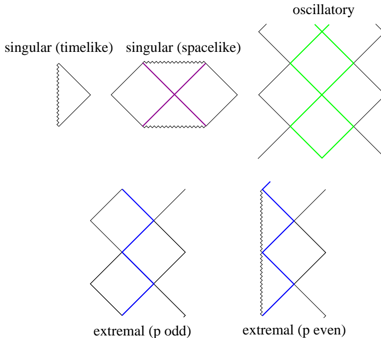
Figure 6. The D -dimensional causal structure of the solutions discussed in the text and shown in figure 5. In the top row, we show the timelike singular (left), spacelike singular (center), and oscillatory (right) solutions generated from an open FRW metric ansatz. In the bottom row are the extremal solutions generated from a flat FRW metric ansatz for p odd (left) and p even (right). Event horizons correspond to the non-singular big-bang and big-crunch surfaces at the stationary points of the p + 2 dimensional cosmological solutions, and are color-coded to correspond to the stationary points in figure 5. Singularities occur when the energy density in \phi diverges at a = 0 , while the asymptotically flat D -dimensional regions are described by the attractor solutions at large \phi .
