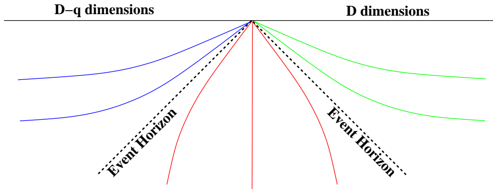
Figure 2. A sketch of the causal structure of a solution that interpolates between asymptotically D - q and D -dimensional regions across event horizons. On the left, a D - q dimensional non-singular cosmological spacetime is located behind an event horizon. Outside this horizon is an interpolating region to another event horizon, that encloses an asymptotically D -dimensional de Sitter region. The nucleation of such solutions from empty D -dimensional de Sitter space represents the dynamical compactification of some number of extra dimensions.
