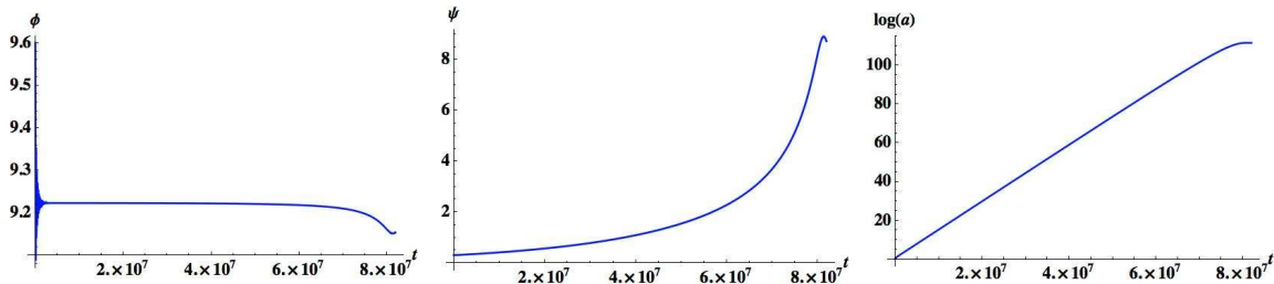
Figure 23. Numerical evolution in the presence of the potential in the left panel of figure 22. The parameters specifying the potential are \{q = 2, n = 6, Q = 142, \Lambda = 5 \times 10^{-5}, \tilde{m} = 3.24 \times 10^{-7}, \xi_1 = 1.63 \times 10^{-3}, \xi_2 = -9 \times 10^{-5}, \lambda = 3.3 \times 10^{-12}\} . The stationary point of the interpolating solution sets the initial condition for \psi to \phi_0 = 9.6 . We choose \psi = .3 to obtain enough inflation (for this initial condition, there are approximately 110 e -folds).
