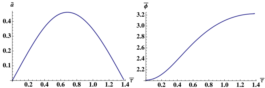
Figure 13. The interpolating solution for p = 2 , q = 2 , Q = 3.2 , and \Lambda/M_D^2 = .1 generated from the initial condition \bar{\phi}_0 \simeq 2.01 . The field interpolates between either side of the potential barrier while the scale factor evolves between its two zeros.
