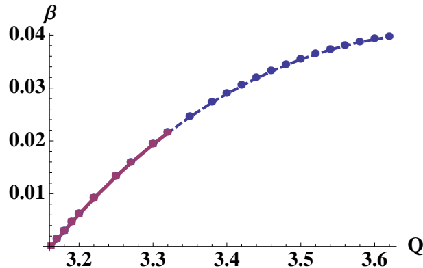
Figure 20. A plot of \beta , the ratio of the instanton action to the p + 2 -dimensional de Sitter action, versus Q for the interpolating (solid line) and compactification (dashed line) solutions with \{p = 2, q = 2, \Lambda = .1\} . The values of \beta are nearly identical for the two solutions. At Q \simeq 3.162 , the minimum of the radion potential goes to zero, sending \beta \rightarrow 0 . The interpolating solution no longer exists for Q > 3.35 , and at the upper range of the plot Q = 3.65 , there are no potential extrema.
