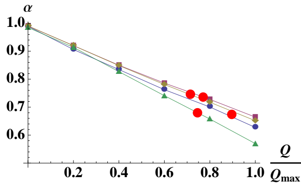
Figure 19. The value of \alpha in D = 8 for p = 1, 2, 3, 4 (blue circles, purple squares, yellow diamonds, and green triangles respectively) versus the normalized charge Q/Q_{\max} . The red circle denotes the value of Q yielding an approximately zero energy p + 2 dimensional vacuum for each p .
