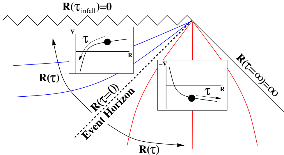
Figure 1. A portion of the causal diagram for a Schwarzschild black hole. To the future of the event horizon, \tau is a timelike coordinate, and the \tau, x plane (which is shown here) resembles a big-crunch cosmology that begins from a completely non-singular “big-bang” at the event horizon. The value of R at the horizon is determined by the stationary point shown on the potential (filled circle). On subsequent surfaces of constant \tau , R evolves in the sketched potential V , eventually reaching a singularity as R is pushed to zero. To the past of the event horizon, \tau \rightarrow i\tau , and \tau becomes a spacelike coordinate. The value of R on surfaces of constant \tau is determined by its motion in the upside-down potential -V . This pushes R \rightarrow \infty as the asymptotically flat region far from the black hole is approached.
