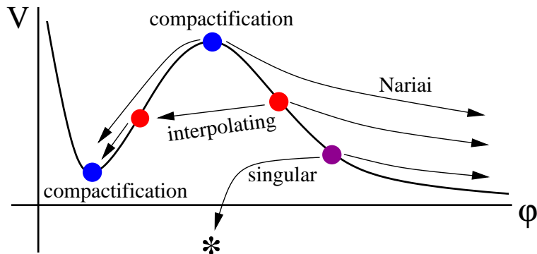
Figure 10. A sketch of the solutions for \Lambda > 0 when the radion potential has a zero or positive energy minimum. There is one de Sitter and one de Sitter or Minkowski compactification solution at the critical points of the potential. As for the case where the radion potential has a negative minimum, for an open FRW ansatz there is an interpolating solution that has two non-singular stationary points connecting the asymptotic \phi \rightarrow \infty region to the basin of attraction of the potential minimum. Motion away from the second stationary point will lead to a completely non-singular evolution towards \phi_- , asymptotically producing a region of p + 2 dimensional Minkowski or de Sitter space. Solutions with any other stationary points contain a timelike singularity. For a flat FRW ansatz, the Nariai solution connects regions interpolating between \phi_+ and \phi_- or \phi \rightarrow \infty over an infinite range in \tau . The Nariai solution is in this case completely non-singular.
