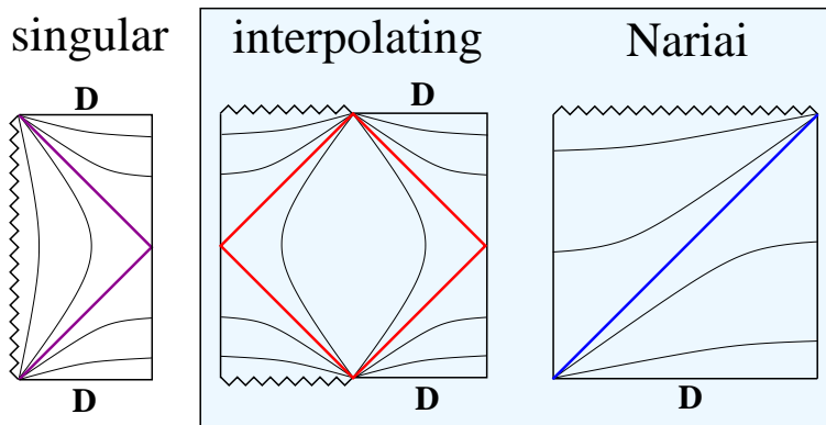
Figure 11. Causal diagrams for \Lambda > 0 solutions with an asymptotically D -dimensional region and a radion potential with a negative minimum. Surfaces of constant \tau are shown as the light solid lines. Starting from the left, we show the singular, interpolating, and Nariai solutions. All solutions contain a timelike or spacelike singularity separated from asymptotically D -dimensional de Sitter space (denoted by the D ) by event horizons. The horizons are in each case color coded with the stationary points of the radion field trajectories in figure 9. We highlight the solutions relevant for dynamical compactification in the shaded box.
