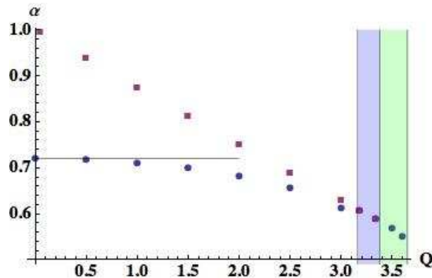
Figure 17. A plot of \alpha versus Q for the Euclidean interpolating (squares) and compactification (circles) solutions with \{p = 2, q = 2, \Lambda = .1\} . The value of \alpha for the compactification solutions approaches the value defined in eq. (6.15) (denoted by the horizontal solid line at \alpha = .72 ) at small Q . A few important thresholds in Q are denoted by the shaded regions. For 3.162 < Q < 3.35 , there exists a minimum of the radion potential that has positive energy. Between 3.162 < Q < 3.35 , in the light (blue) shaded region, both the Euclidean interpolating and compactification solutions are allowed. For 3.35 < Q < 3.65 , in the dark (green) shaded region, only the Euclidean compactification solution exists. When it exists, the interpolating solution always makes the dominant contribution to the decay rate.
