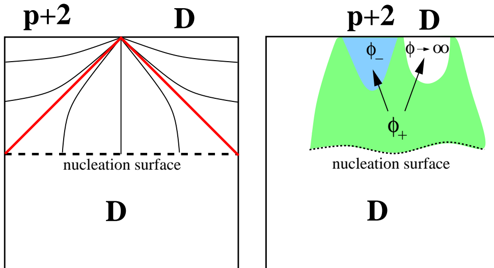
Figure 15. The spacetime picture of dynamical compactification when it is mediated by the Euclidean interpolating (left) and compactification (right) solutions. On the left, the initial D -dimensional de Sitter space is matched across the nucleation surface to the interpolating solution of section 5. The surfaces of constant \phi are shown as solid lines, and interpolate across the barrier of the radion potential along the nucleation surface. On the right, roughly a horizon-volume of the initial D -dimensional de Sitter space fluctuates to the compactification solution at the maximum of the radion potential. After the fluctuation, the radion falls from its unstable equilibrium in different spacetime regions, producing pockets where the field either evolves to the minimum of the radion potential or off to infinity where the q -sphere decompactifies.
