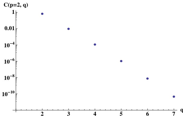
Figure 21. A log plot of the function C(p, q) for p = 2 and various q , obtained numerically by finding the value of the potential minimum for values of Q that yield V_0 \sim 0 , constructing the function V(\phi_-[Q]) , evaluating the derivative, and factoring out the scaling with \Lambda determined in eq. (7.5). It can be seen that the behavior is approximately exponential in q .
